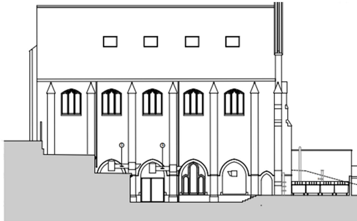
North Sectional Elevation 1:100
